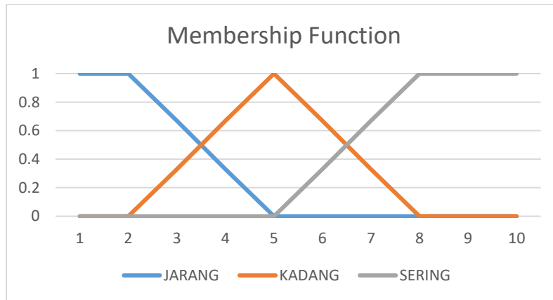
Figure 2. Membership function graph
